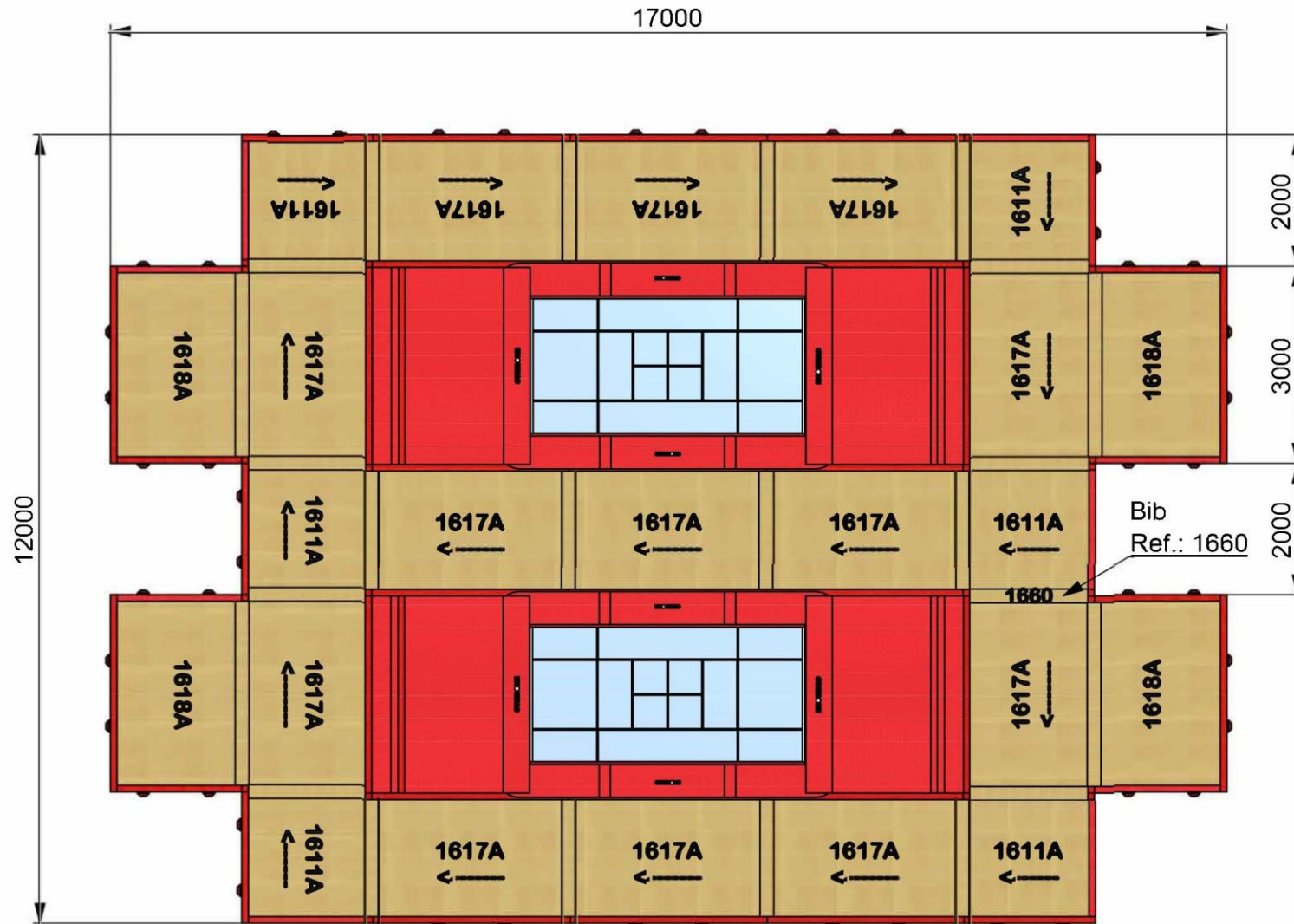
REF. 1785 - Set of FIG mats for safety area for 2 Trampolines (6 Ref. : 1611, 13 ref.: 1617, 4 ref.: 1618, 1 ref.: 1660)
