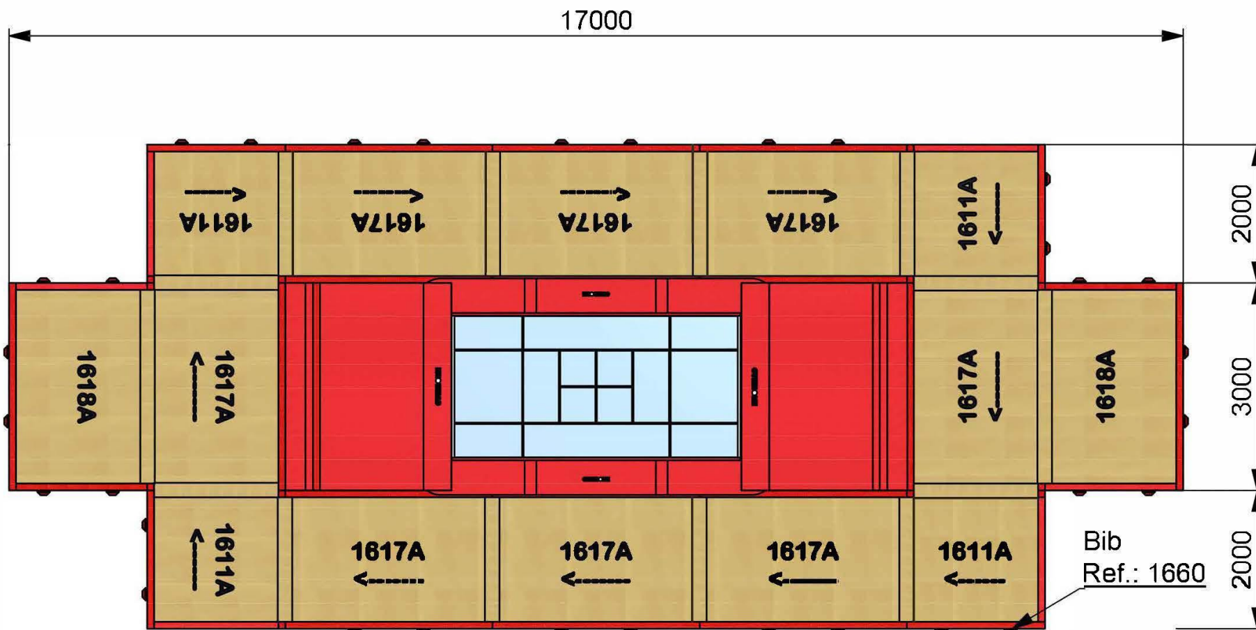
REF. 1780 - Set of FIG mats for safety area for 1 trampoline (4 Ref. : 1611, 8 ref.: 1617, 2 ref.: 1618)
