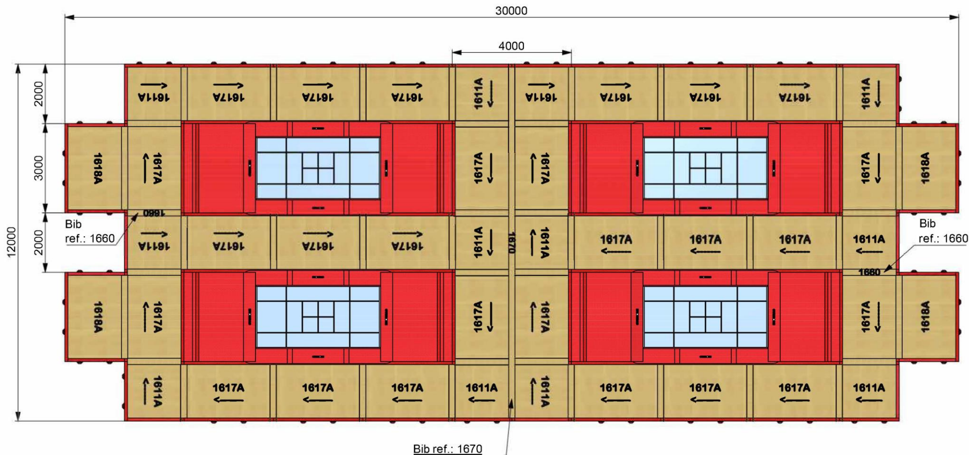
REF. 1790 - Set of FIG mats for safety area for 4 Trampolines (12 Ref. : 1611, 26 ref.: 1617, 4 ref.: 1618, 2 ref.: 1660, 1 ref.: 1670)
